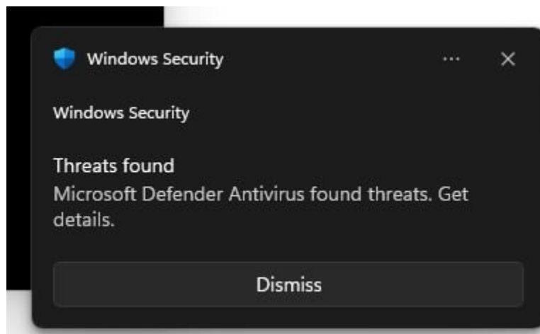
Windows Security
